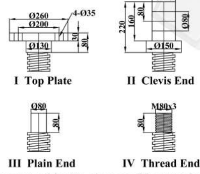
Screw End Types and Dimensions
