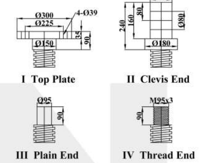
Screw End Types and Dimensions
