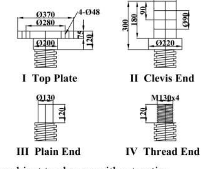
Screw End Types and Dimensions
